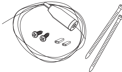
SA NCR19 Component Kit Steel Wire, Crimping Tubes, Screw, Cable ties SA 95A6
